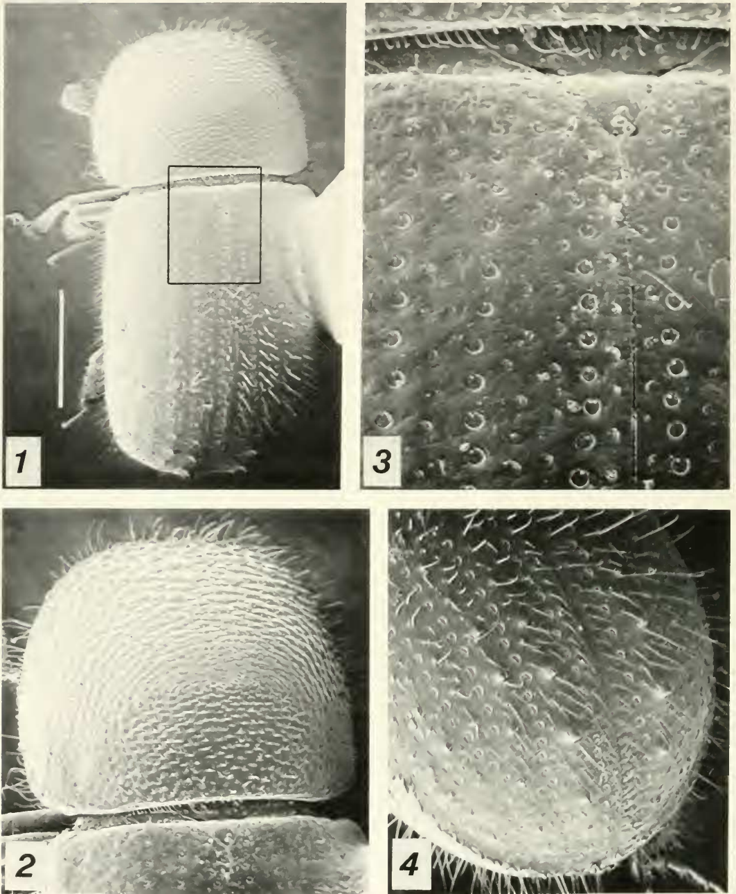
Figs. 1-4. Scanning electron micrographs, Ambrosiodmus lewisi . 1, female, dorsal aspect, 23.4\times (highlighted area magnified in Fig. 3); scale line = 1.0 mm. 2, pronotum, 47.4\times . 3, closeup of surface of left elytron (note irregular double row of fine punctures of interstriae 2 and 3), 117\times . 4, declivity, 57\times .
